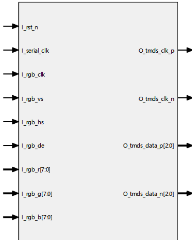
Figure 3-5 DVI TX I/O Diagram
