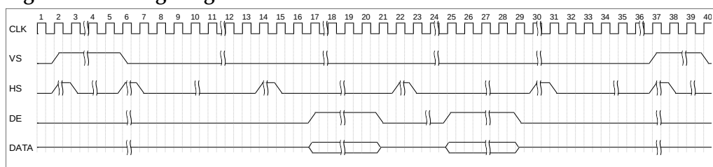
Figure 3-7 Timing Diagram of DVI
