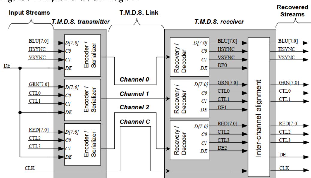
Figure 3-2 Implementation Diagram
