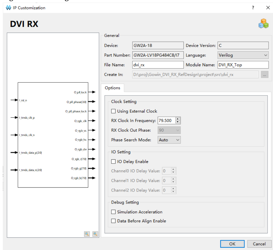
Figure 4-8 Port Diagram of DVI RX IP
